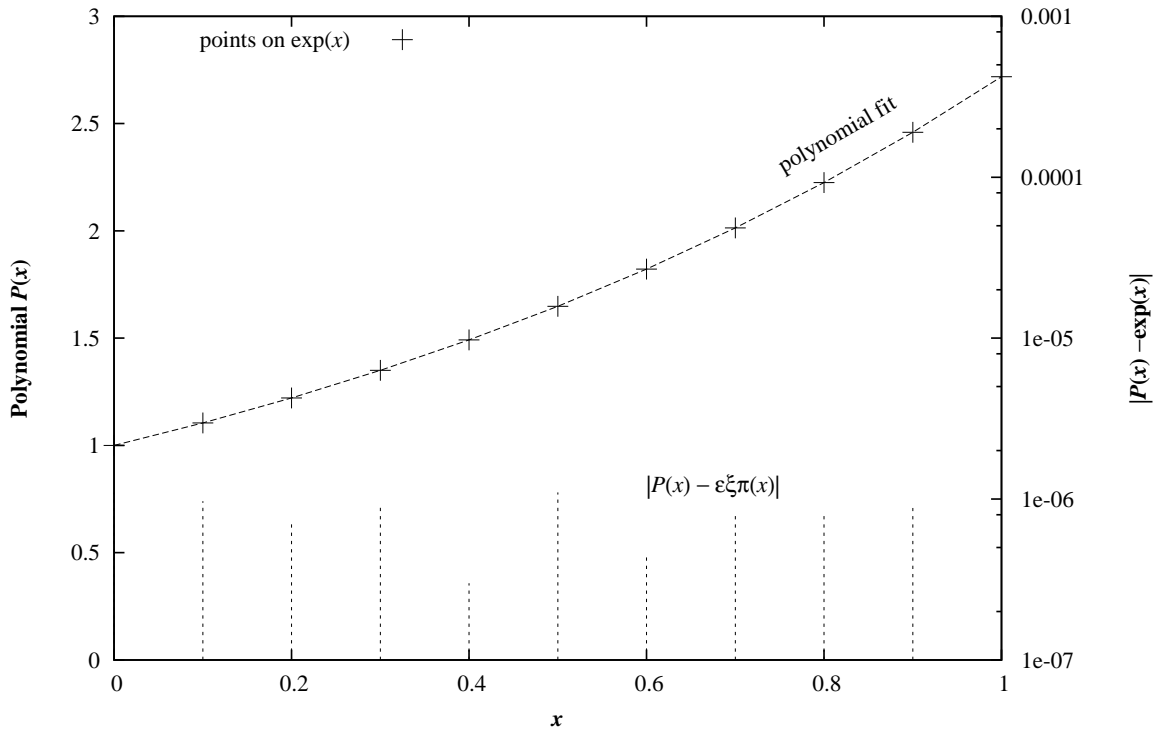
Example Program Minimax Fit to the Exponential Function on the Interval [0,1] using a Degree Five Polynomial, P(x) , given \exp(x) Evaluated at 21 Points
