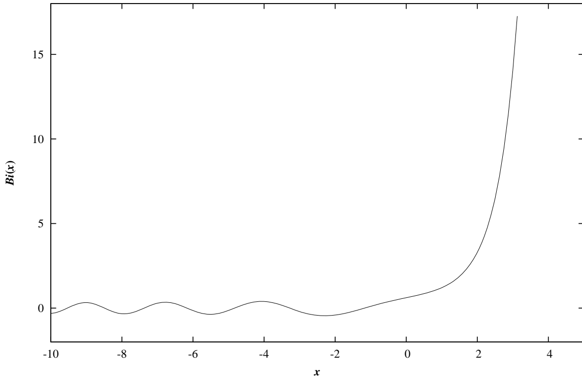
Example Program Returns a Value of the Airy Function Bi(x)
