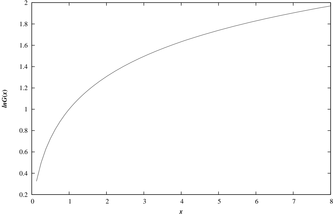
Example Program Returns the Value of \ln G(x) , the Scaled Logarithm of the Gamma Function \Gamma(x)
