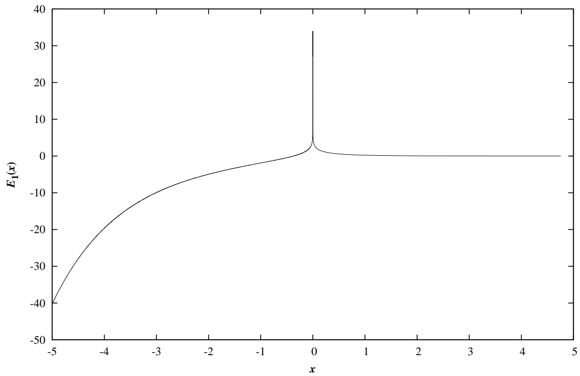
Example Program Returned Values for the Exponential Integral E_1(x)
