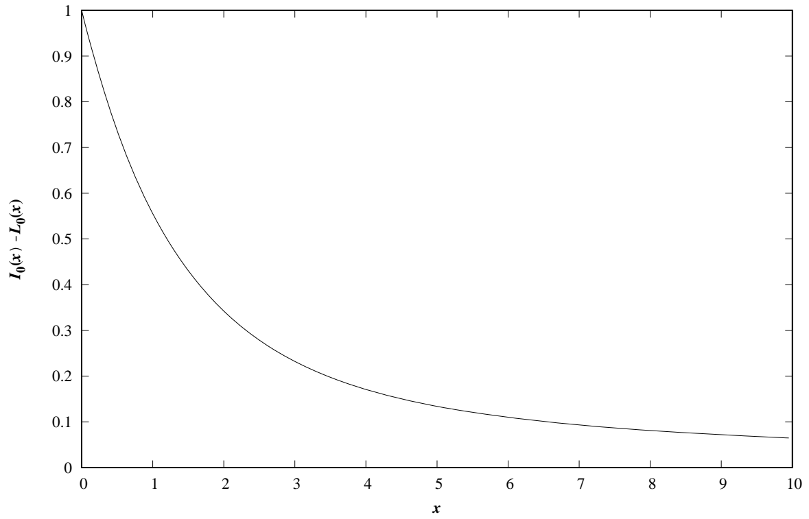
Example Program Returns values for the Bessel Function - the modified Struve Function I_0(x)-L_0(x)
