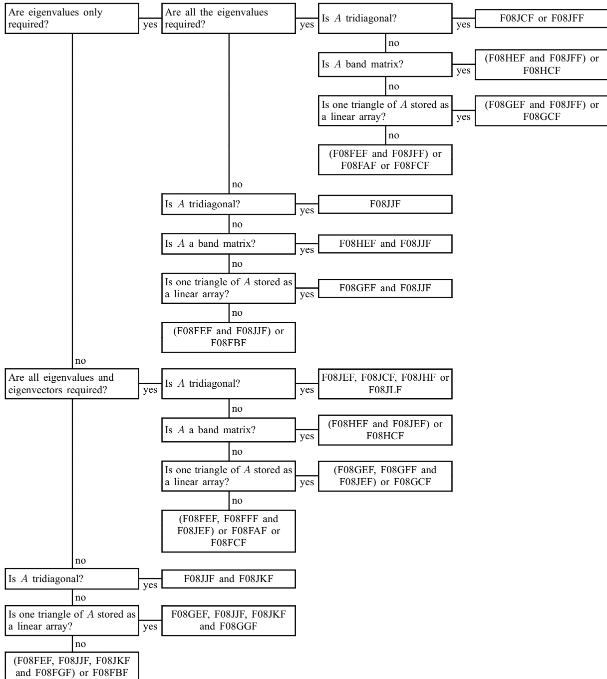
Tree 1: Real Symmetric Eigenvalue Problems
