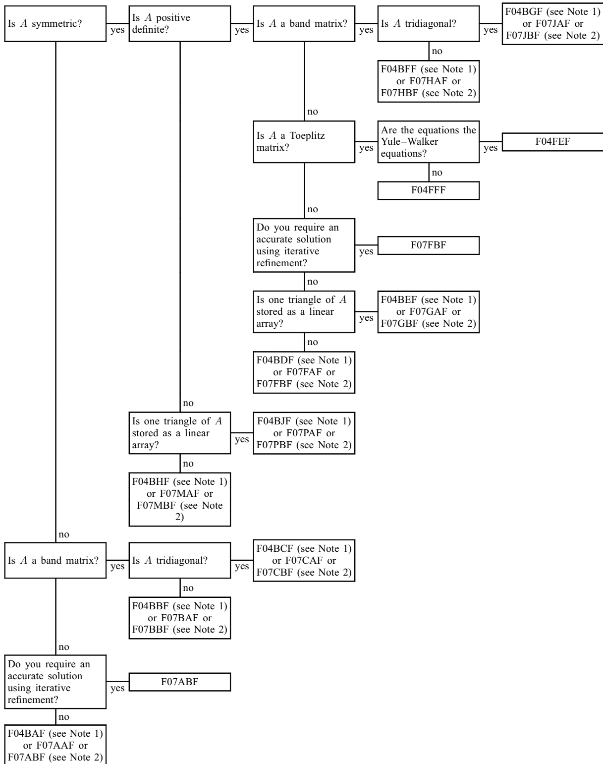
Tree 1: Black Box routines for unique solution of Ax = b (Real matrix)
