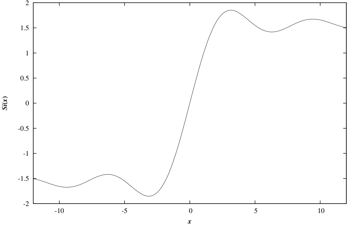
Example Program Returned Values for the Sine Integral Si(x)
