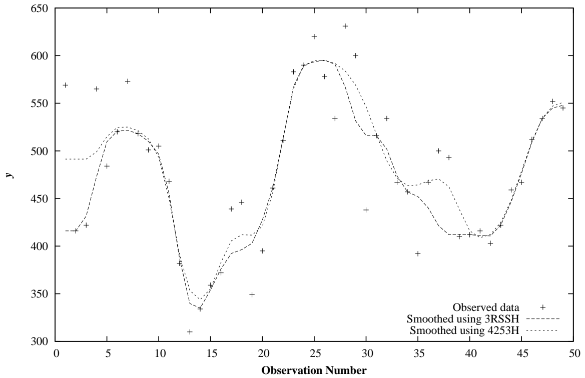
Example Program Running Median Smoothers
