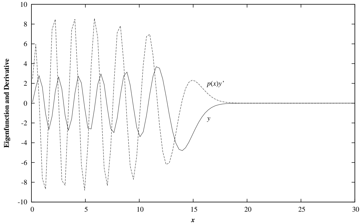
Example Program Regular Singular Second-order Sturm-Liouville System 11th Eigenfunction and Derivative
