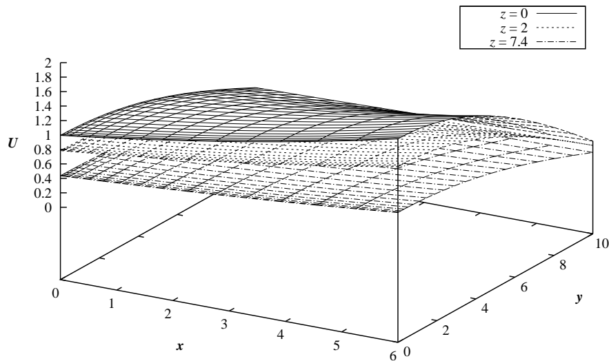
Example Program Solution of Three-dimensional Laplace's Equation in a Box Solutions in the xy -plane for Various Values of z
