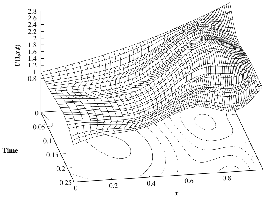
Solution of First-order System using Moving Mesh U(2,x,t)
