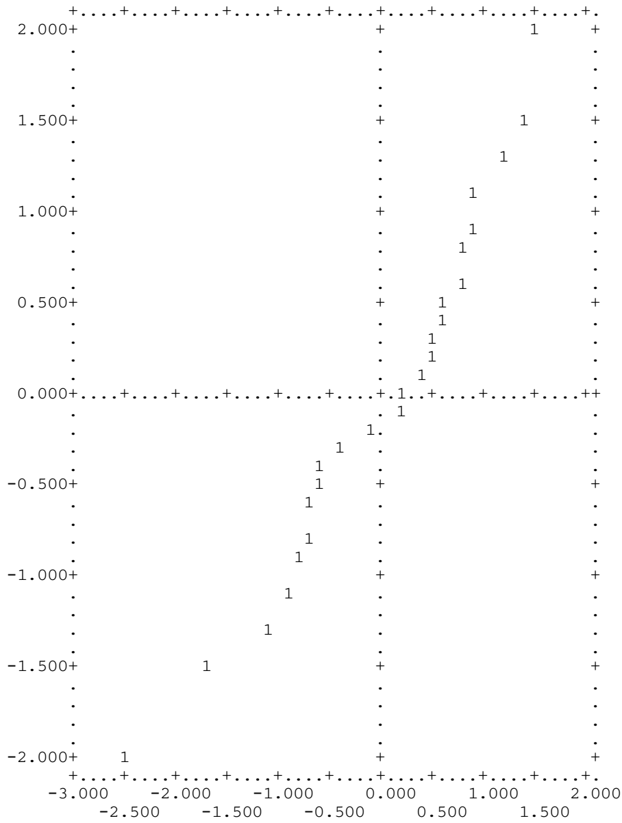
Plot of normal scores (Y) against standardised residuals (X)
