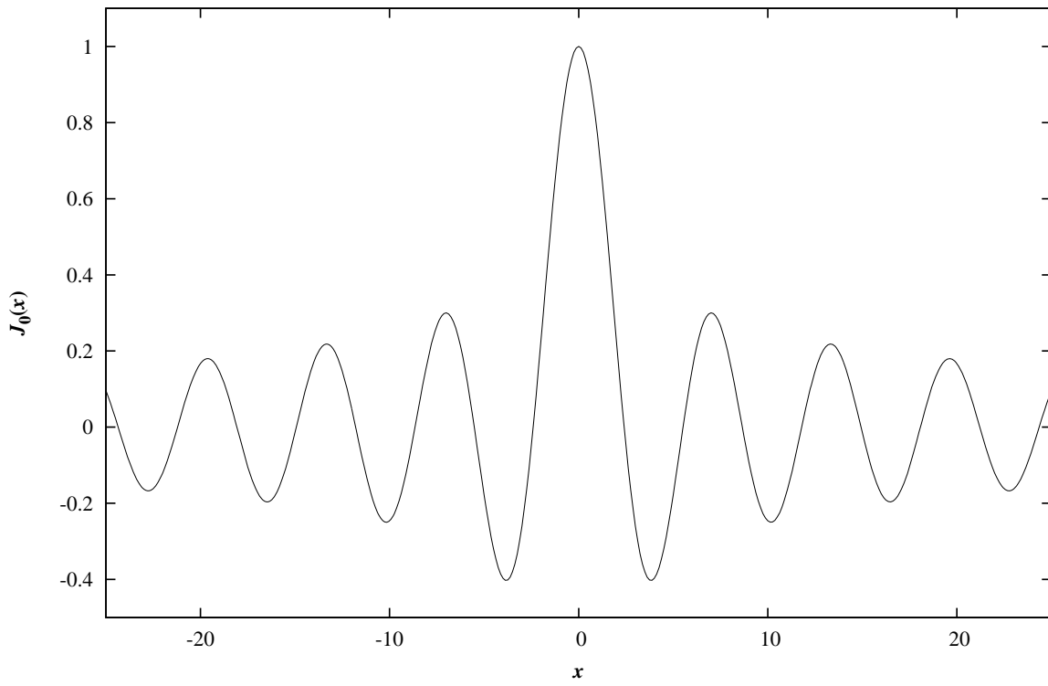
Example Program Returned Values for the Bessel Function J_0(x)
