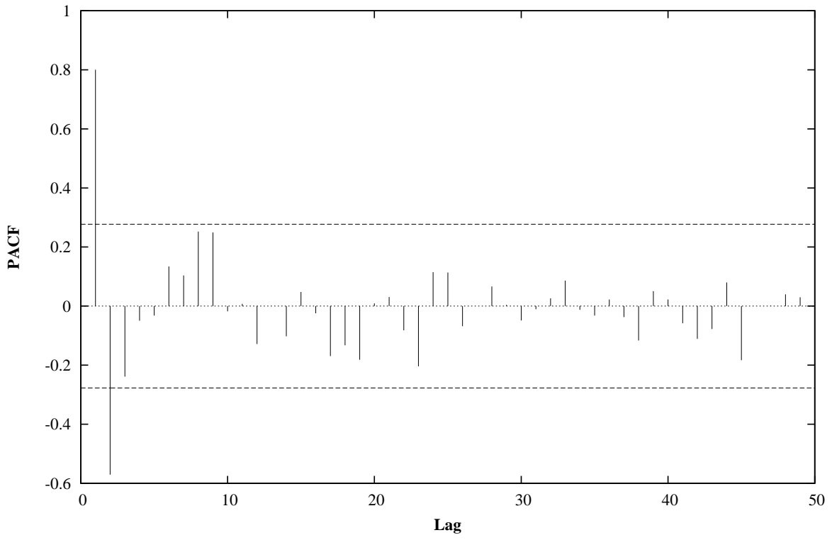
Example Program Partial Autocorrelation Coefficients
