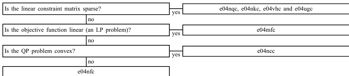
Tree 3: Linear and Quadratic Programming (LP and QP)
