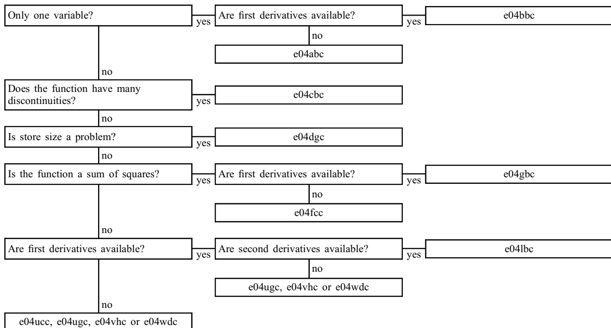
Tree 1: Selection chart for unconstrained problems
